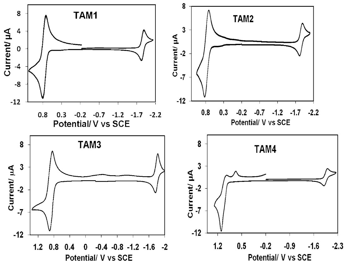
Figure 2. Cyclic voltammograms of TAM1 – TAM4 in 1:1 Bz:MeCN, 0.1 M Bu 4 NPF 6 , scan rates 100 mV/s. Working electrode: Pt inlaid disk (diameter ~ 0.5 mm), counter electrode: Pt coil, reference electrode: Ag QRE.
