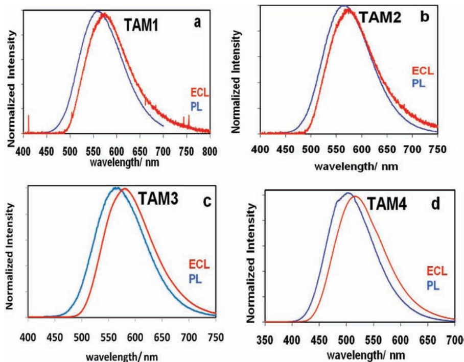
Figure 6. ECL and PL spectra for the 1 mM star-shaped molecules in 1:1 MeCN:Bz, 0.1 M Bu 4 NPF 6 as a supporting electrolyte. TAM1–TAM3 are direct annihilation ECL ( E_{pc} - 80 mV and E_{pa} + 80 mV). TAM4 is coreactant ECL using 10 mM BPO. WE is J-type \sim 2 mm platinum electrode, RE is Ag wire as a quasireference electrode, CE is Pt coil.
